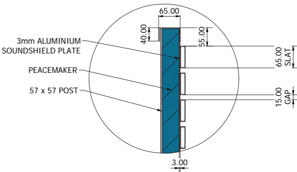
ClassicScreen Wall with Acoustic+
