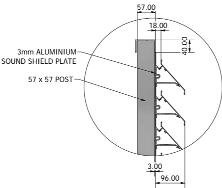
LouvreWall airflow and Soundshield
