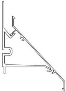
A (1:10) POWDERCOATED WEATHER LV-100 LOUVRE
